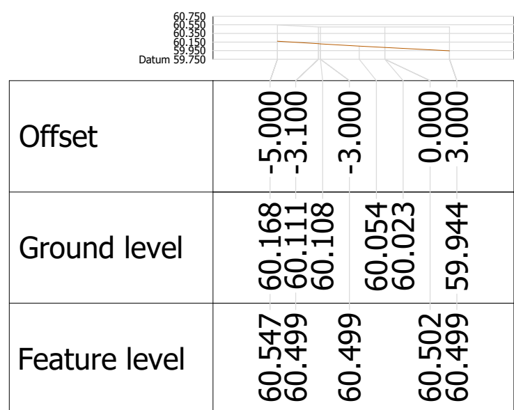
Alignment ARTERIAL Chainage 190.000
