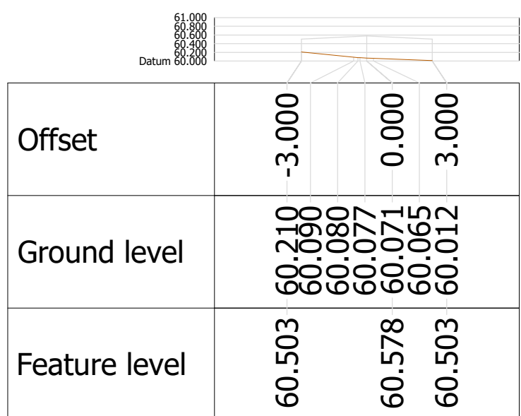
Alignment ARTERIAL Chainage 210.000
