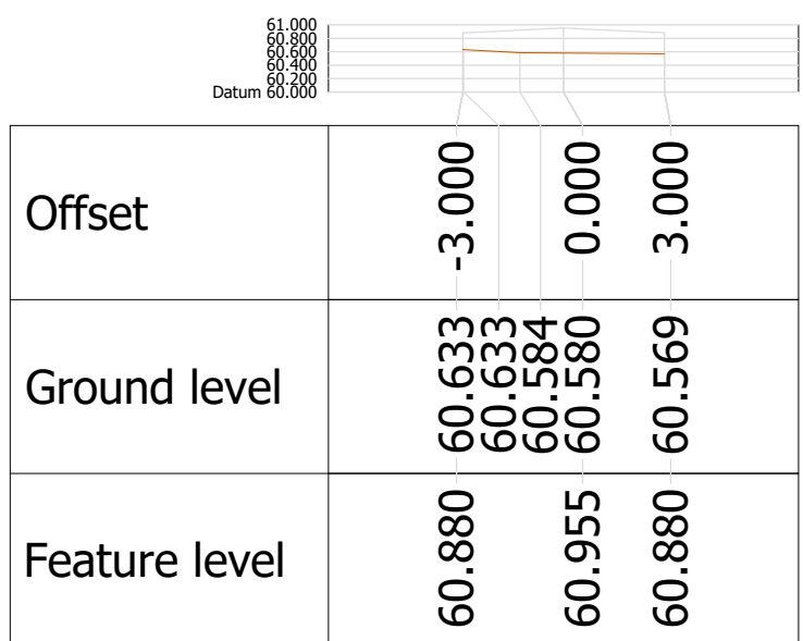
Alignment ARTERIAL Chainage 240.000
