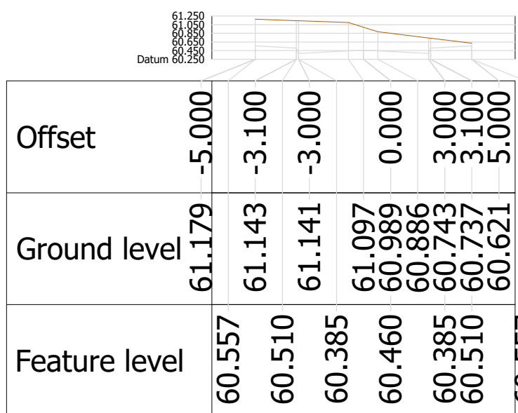
Alignment ARTERIAL Chainage 120.000
