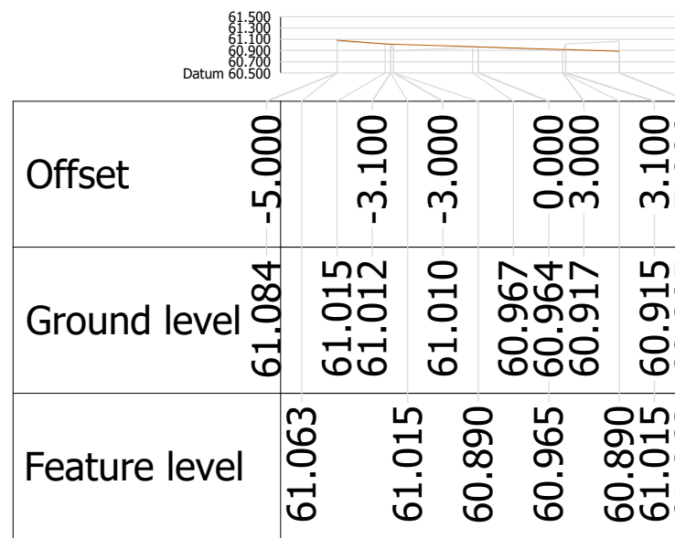
Alignment ARTERIAL Chainage 80.000
