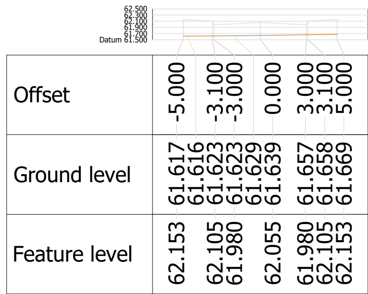
Alignment ARTERIAL Chainage 10.000
