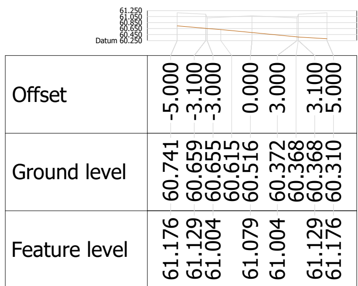
Alignment ARTERIAL Chainage 150.000
