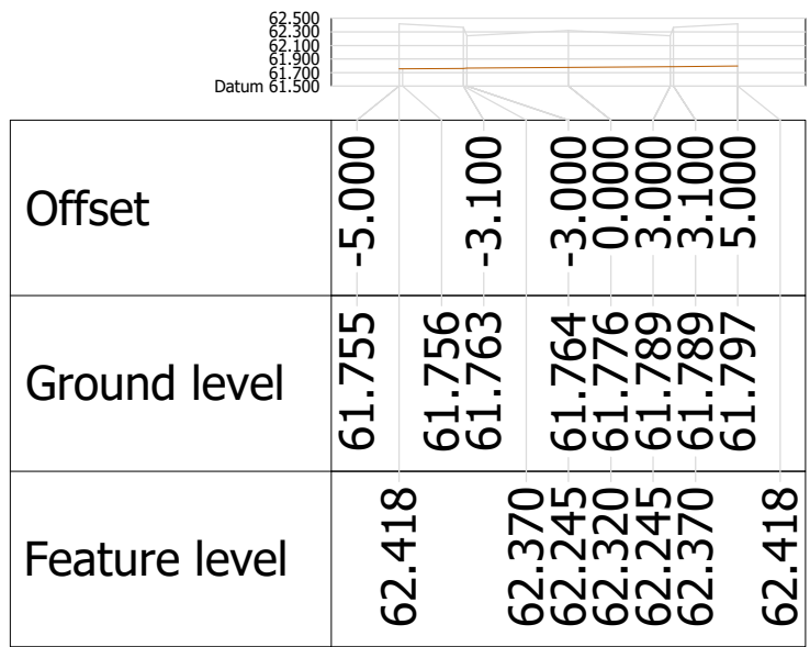
Alignment ARTERIAL Chainage 0.000
