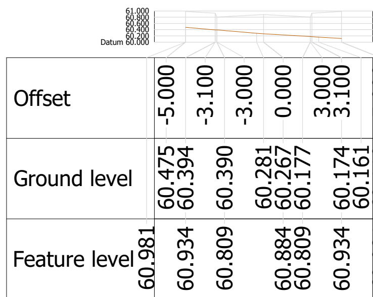
Alignment ARTERIAL Chainage 160.000
