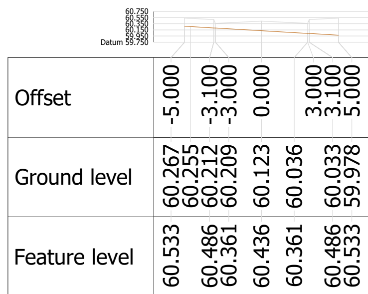
Alignment ARTERIAL Chainage 170.000
