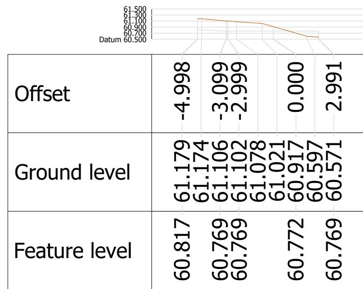
Alignment ARTERIAL Chainage 110.000
