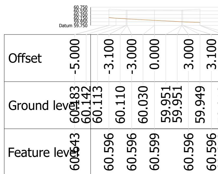
Alignment ARTERIAL Chainage 200.000
