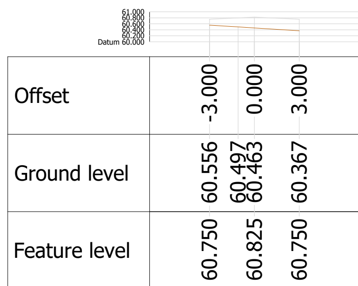
Alignment ARTERIAL Chainage 230.000
