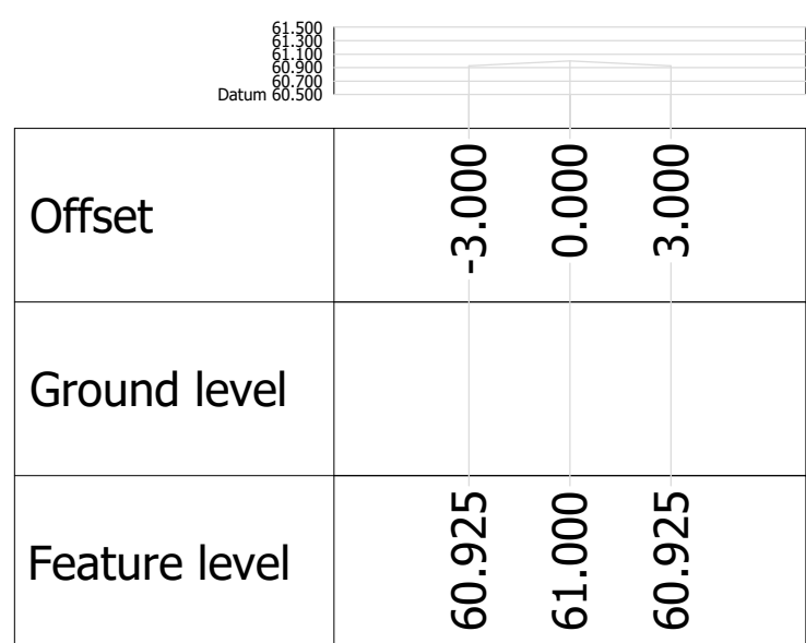
Alignment ARTERIAL Chainage 243.415
