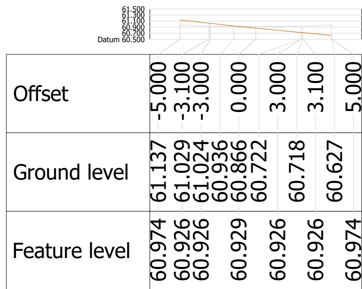
Alignment ARTERIAL Chainage 100.000
