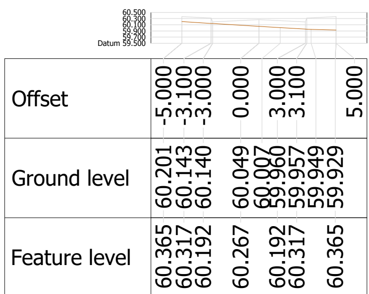
Alignment ARTERIAL Chainage 180.000
