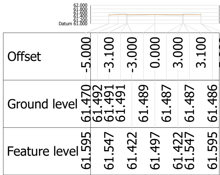
Alignment ARTERIAL Chainage 30.000
