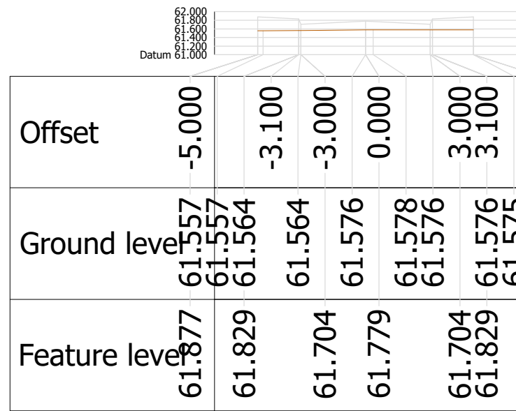
Alignment ARTERIAL Chainage 20.000
