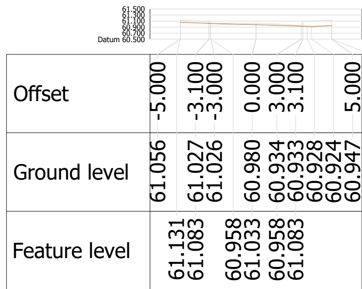
Alignment ARTERIAL Chainage 70.000
