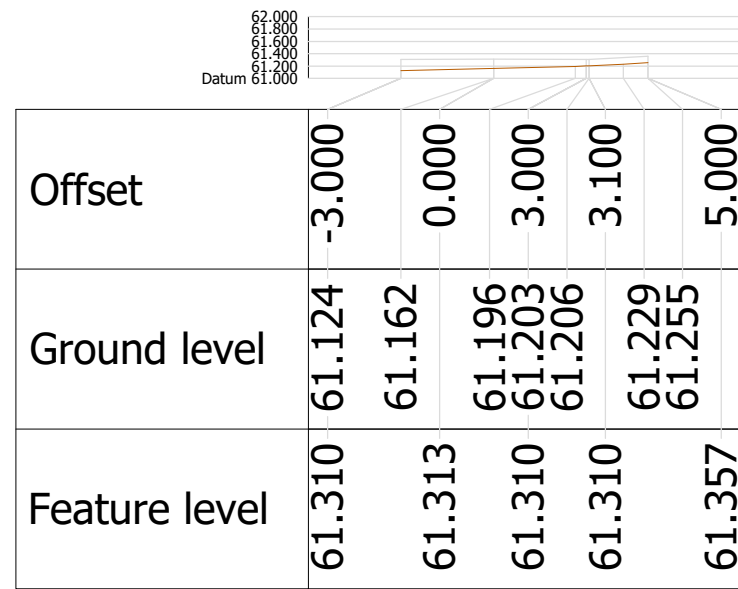
Alignment ARTERIAL Chainage 50.000
