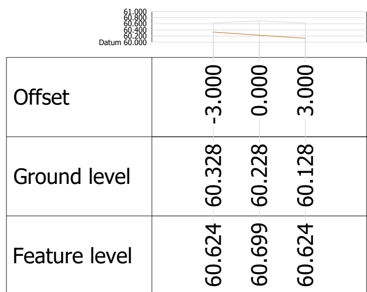
Alignment ARTERIAL Chainage 220.000
