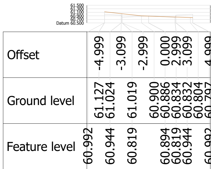
Alignment ARTERIAL Chainage 90.000
