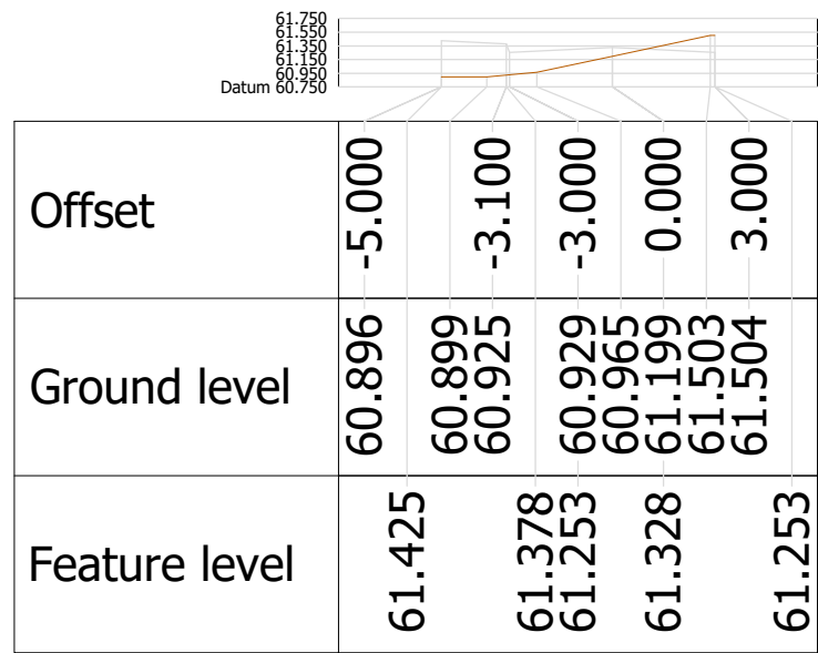
Alignment ARTERIAL Chainage 40.000
