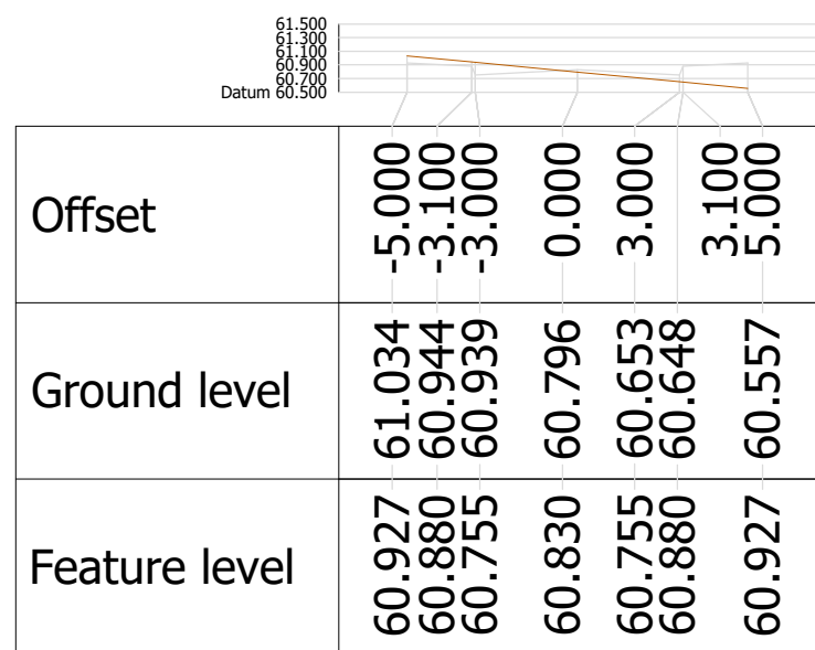
Alignment ARTERIAL Chainage 140.000
