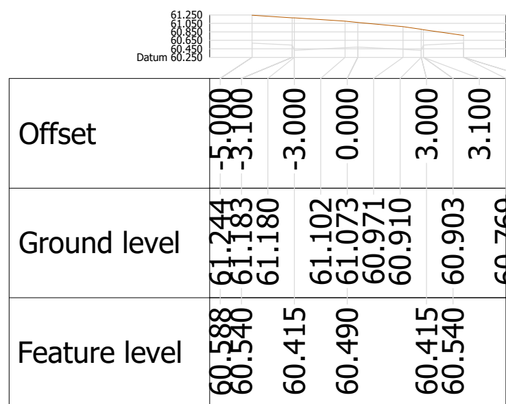
Alignment ARTERIAL Chainage 130.000
