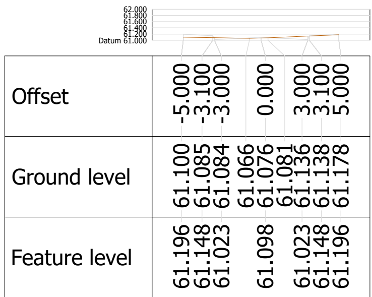
Alignment ARTERIAL Chainage 60.000
